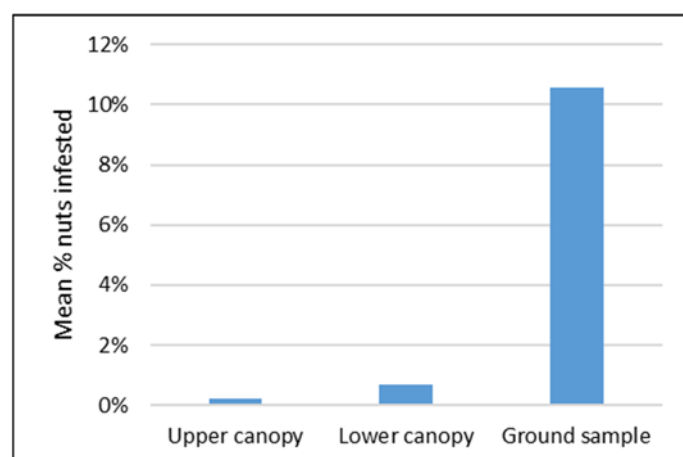
Figure 2. Variation in infestation of almond mummy nuts with live carpophilus beetle in winter, between various sampling positions.
