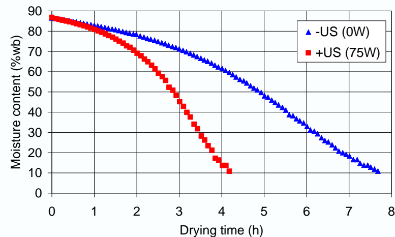
Effect of ultrasound on drying kinetics of apple ( T=40^{\circ}\text{C} ; \text{RH}=25\% ; V=1.0\text{m/s} ; 5mm slices).
