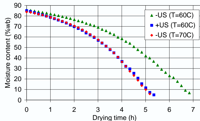
Effect of ultrasound on drying kinetics of apple (US Power=75W; \text{RH}=25\% ; V=1.0\text{m/s} ; 5mm slices).
